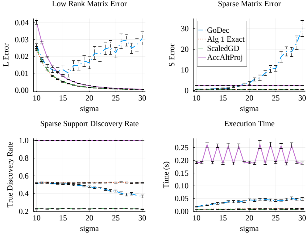
Figure 3: Low-rank matrix reconstruction error (top left), sparse matrix reconstruction error (top right), sparse support discovery rate (bottom left) and execution time (bottom right) versus \sigma with n = 100 , k_0 = 5 and k_1 = 500 . Averaged over 50 trials for each parameter configuration.
