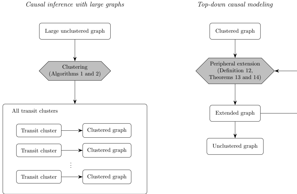
Figure 2: A schematic illustration of the contributions of the paper. In causal inference with large graphs (left), the application of the proposed clustering algorithm to a large graph results in a collection of all transit clusters, each of which corresponds to a clustered graph. In top-down causal modeling (right), we start with a clustered graph and iteratively apply peripheral extension to obtain an unclustered graph that shares the key properties with the clustered graph.
