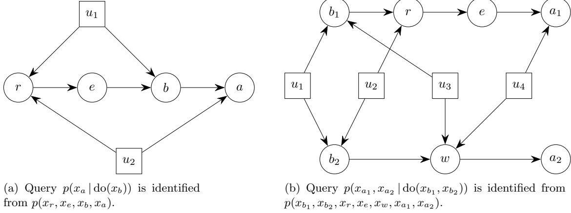
Figure 4: Two examples where identifiability is lost when transit cluster T = \{r, e\} is replaced by a single vertex. The vertices of unobserved variables are denoted by squares.
