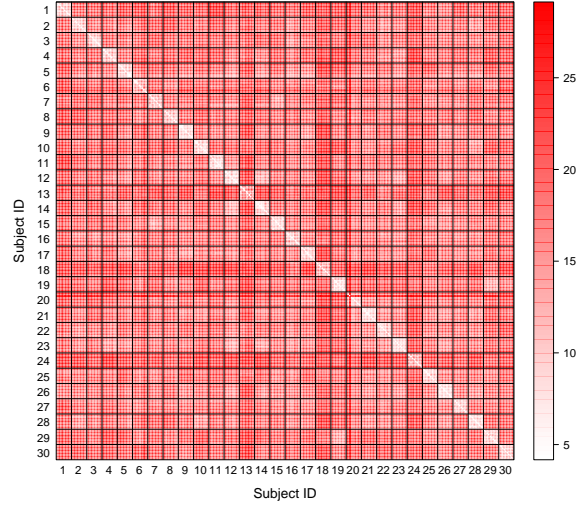
Figure 12: Matrix of distances between the estimated score parameters. Each entry of the matrix corresponds to the distance between the MASE estimated score matrices of a pair of graphs from the HNU1 data, composed by 30 subjects with 10 graphs each. Distances between graphs of the same subject are usually smaller than distances between different subjects.
