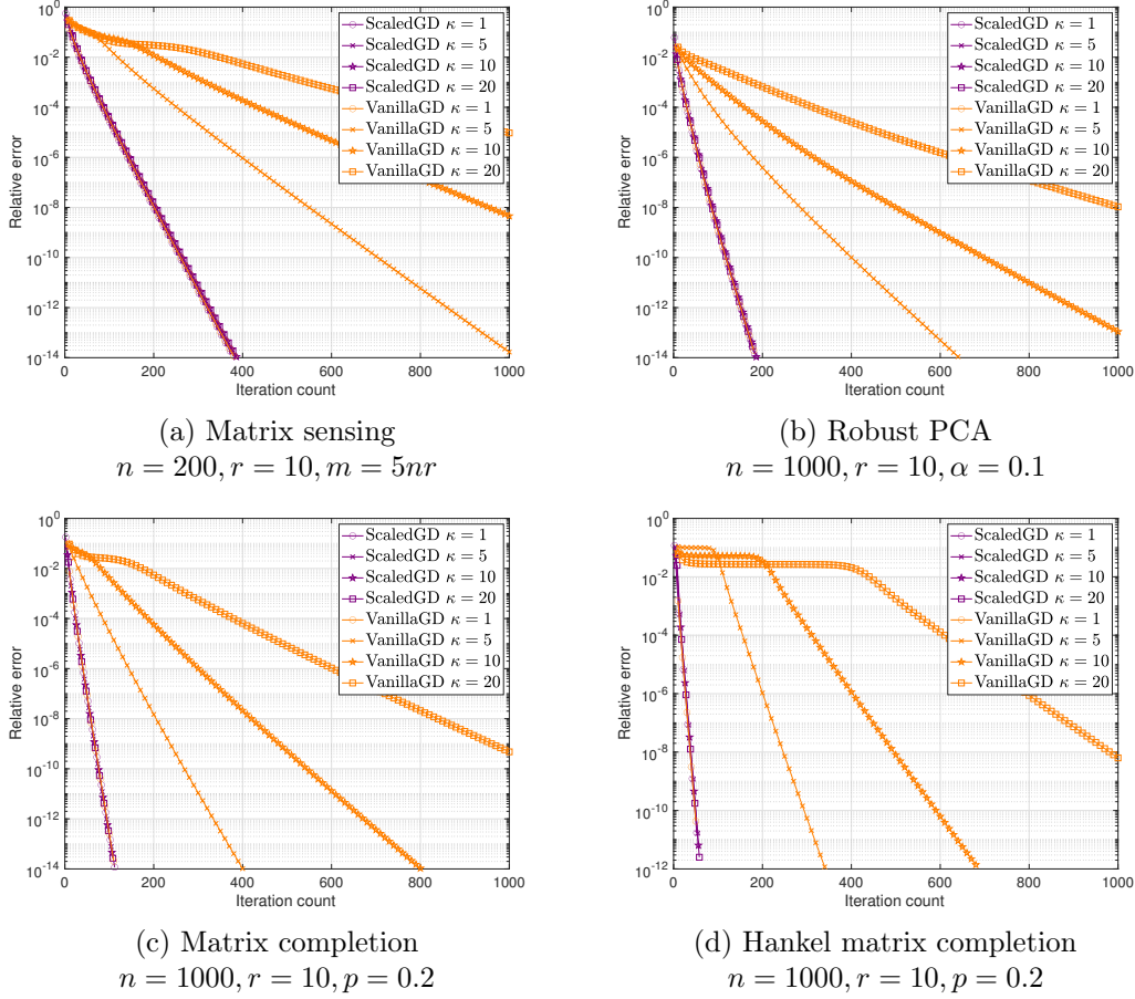
Figure 2: The relative errors of ScaledGD and vanilla GD with respect to the iteration count under different condition numbers \kappa = 1, 5, 10, 20 for (a) matrix sensing, (b) robust PCA, (c) matrix completion, and (d) Hankel matrix completion.
