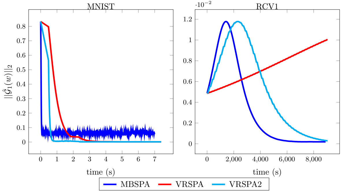
Figure 2: Bound on subdifferential mapping of algorithms of this paper on datasets MNIST and RCV1.
