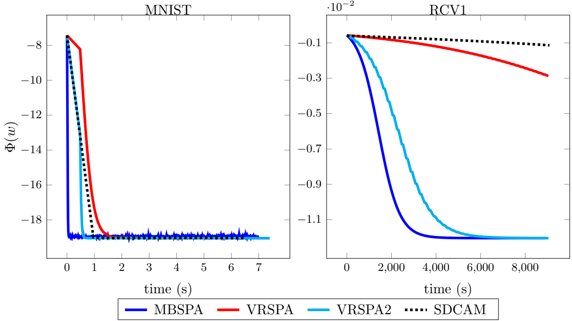
Figure 1: Comparison of algorithms of this paper and SDCAM (Liu et al., 2019) on datasets MNIST and RCV1.
