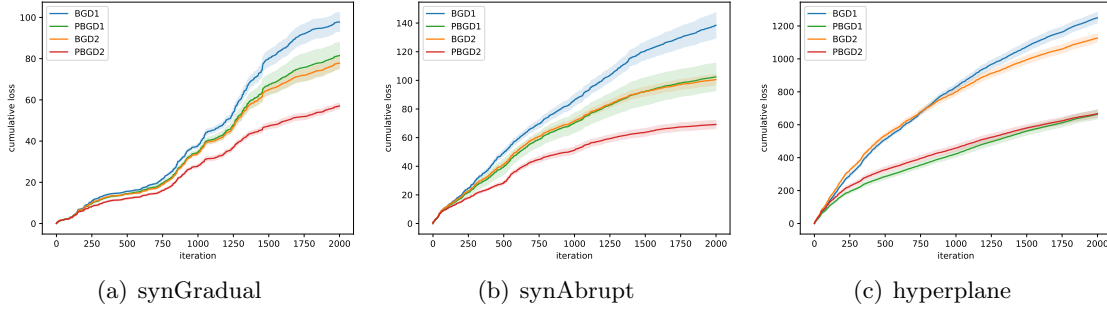
Figure 1: Cumulative loss of BGD and PBGD on three synthetic datasets: synGradual, synAbrupt, and hyperplane. BGD1/PBGD1 denotes the methods for BCO with one-point feedback, and BGD2/PBGD2 denotes the methods for BCO with two-point feedback.
