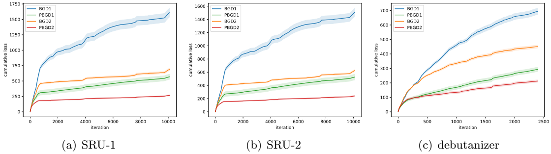
Figure 2: Cumulative loss of BGD and PBGD on three real-world datasets: SRU-1, SRU-2, and debutanizer. BGD1/PBGD1 denotes the methods for BCO with one-point feedback, and BGD2/PBGD2 denotes the methods for BCO with two-point feedback.
