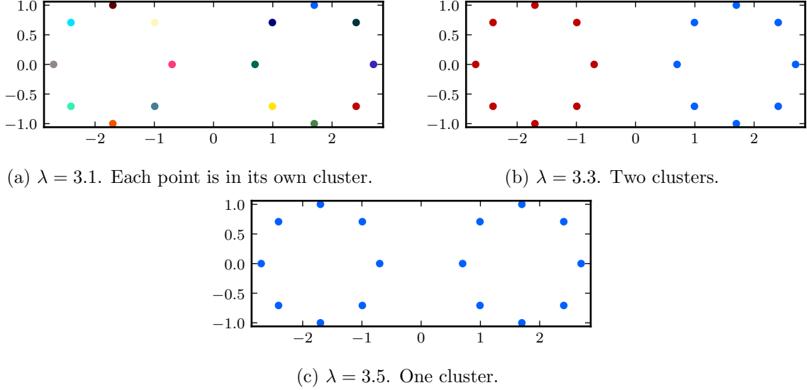
Figure 3.1: Clustering results for the vertices of two octagons. Vertices assigned to the same cluster are drawn in the same color.
