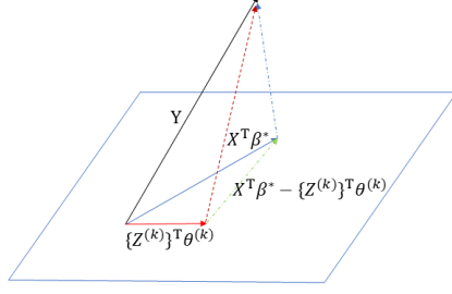
Figure 2: Projection of Y \in \mathbb{R} on the space of all linear combinations of X \in \mathbb{R}^p . Here, Z^{(k)} \in \mathbb{R}^{p_k} is a subvector of X for k = 1, \dots, K .
