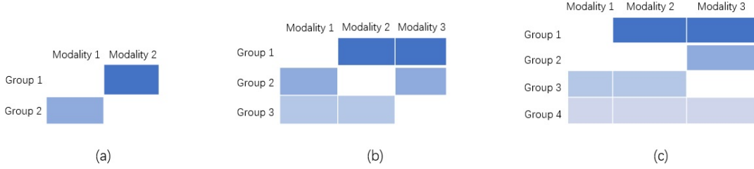
Figure 1: Different structures of block-missing data. Each blank block represents the missingness of a certain modality.
