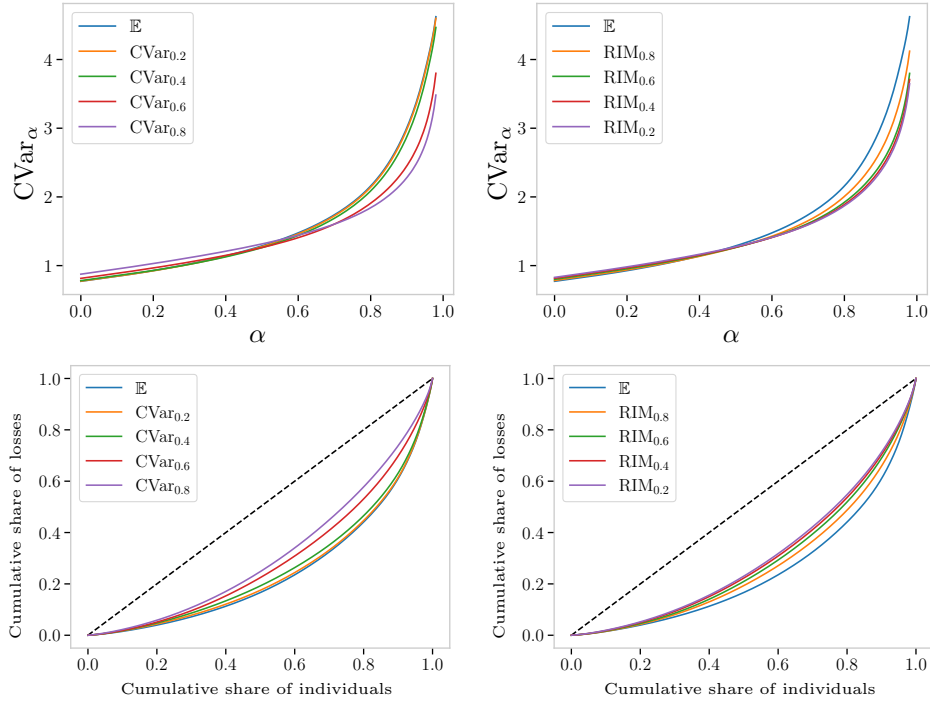
Figure 9: PCA* results on adult . Top row: \text{CVar}_\alpha curves of test losses for \text{CVar}_\alpha risk measures (left) with different \alpha and RIMs risk measures (right) with different \beta , indicated by subscript, where \alpha = 0.7 . For better visibility of the differences, we cut off \alpha at 0.98. Bottom row: Lorenz curves of test losses for \text{CVar}_\alpha (left) and RIMs (right) with \alpha = 0.7 and different \beta .
