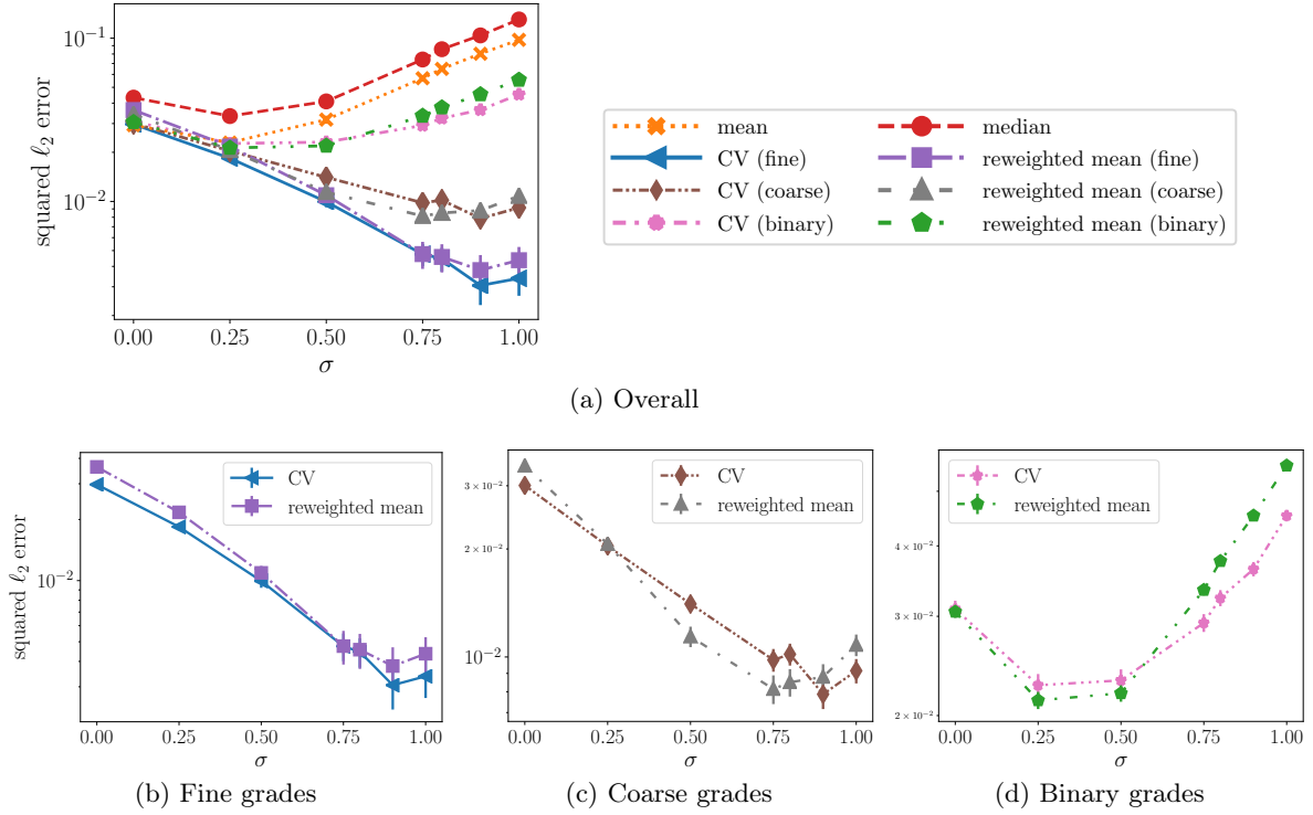
Figure 5: The performance of our estimator (with cross-validation) on semi-synthetic grading data, compared to the mean, median and reweighted mean estimators.
