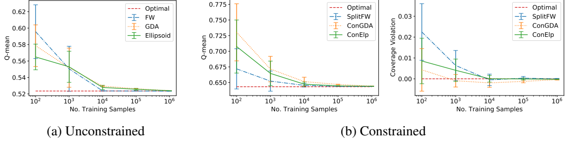
Figure 7: Convergence of the proposed algorithms on synthetic data to (a) the Bayes optimal classifier for the Q-mean loss, and (b) the optimal-feasible classifier for the task of minimizing Q-mean loss subject to a coverage constraint, with the Q-mean loss shown on the left and the coverage constraint violation \max_{i \in [3]} |\sum_j C_{ji} - \pi_i| - 0.01 shown on the right. The results are reported on the test set, and averaged over training with 5 random draws of the dataset.
