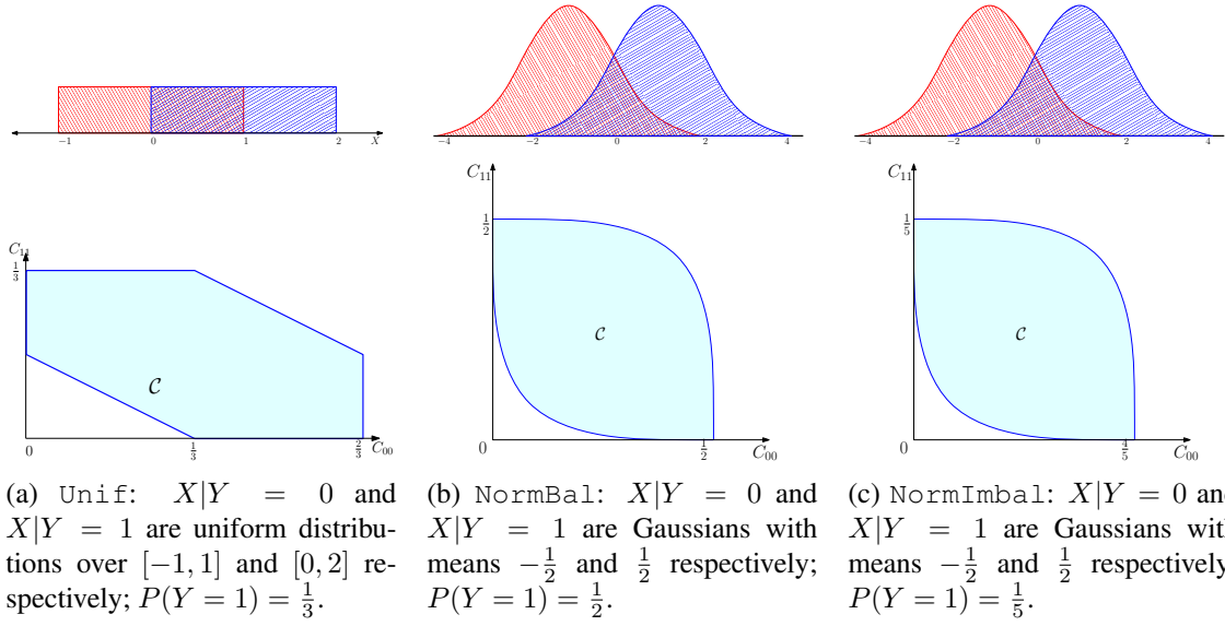
Figure 2: The set of achievable confusion matrices \mathcal{C} for three example binary-labeled distributions: (a) Unif, (b) NormBal, and (c) NormImbal. The top row figures show the class-conditional distributions, and the bottom row figures represent the corresponding \mathcal{C} . While the confusion matrix has four entries, there are only two degrees of freedom (the rows of the confusion matrix sum to the prior probabilities). We therefore only illustrate the projection of \mathcal{C} on to the diagonal entries C_{00} and C_{11} . Note that the scales in the bottom row figures are different.
