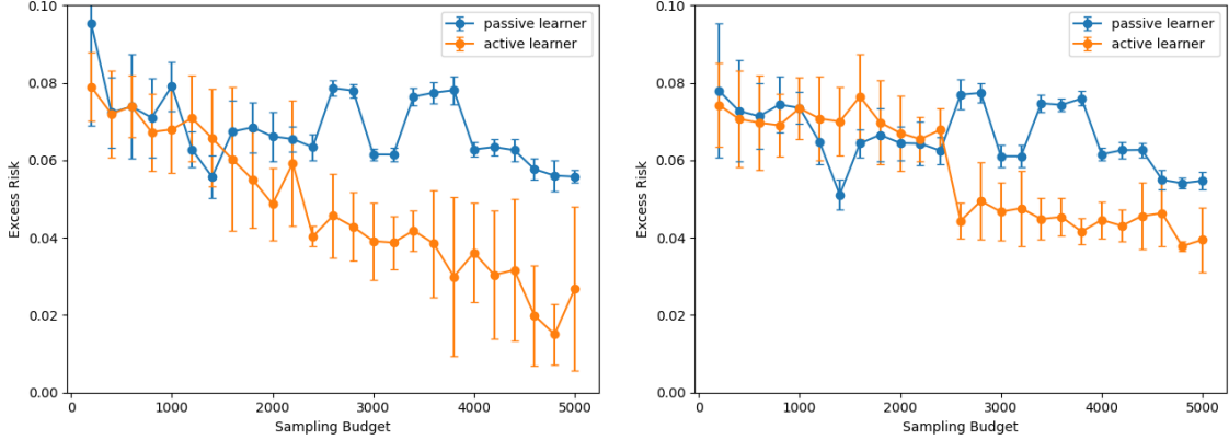
Figure 4: The empirical excess risk of the active learner and passive learner versus the sampling budget, for \varepsilon_0 = 0 (left) and \varepsilon_0 = 0.6 (right). Each dot represents the mean empirical excess risk over 10 replications, and the error bars stand for the standard deviation.
