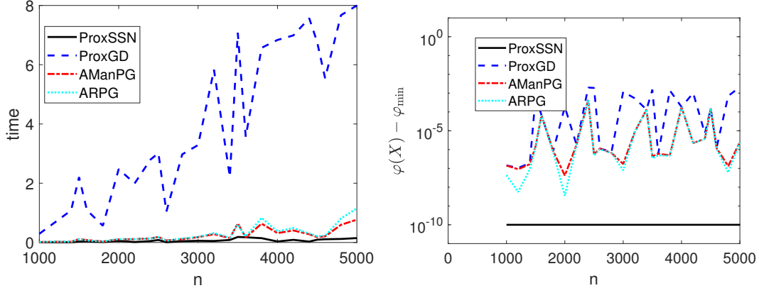
Figure 6: Comparisons of wall-clock time and the objective function values on the sparse least square regression (8) with m = 30 , \lambda = 0.01 for different n .
