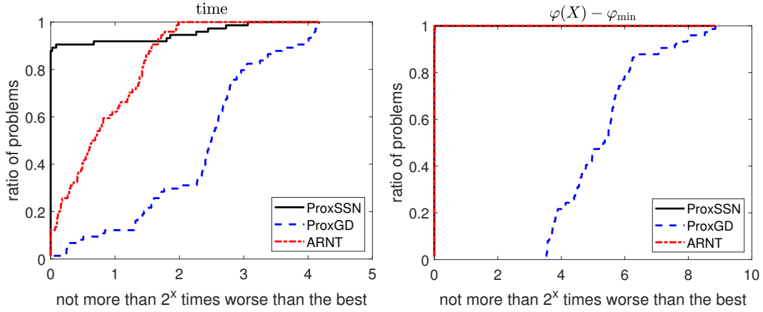
Figure 11: The performance profiles on the BEC problem (39).
