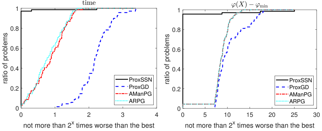
Figure 4: The performance profiles on the sparse PCA problem (3).
