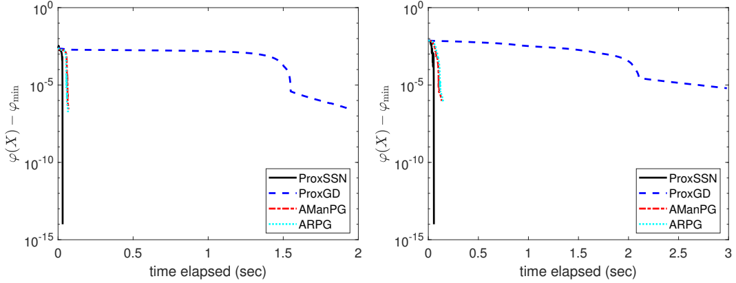
Figure 5: The trajectories of the objective function values with respect to the wall-clock time on the sparse least square regression (8) with m = 20, \lambda = 0.01 . Left: n = 2000 ; right: n = 3000 .
