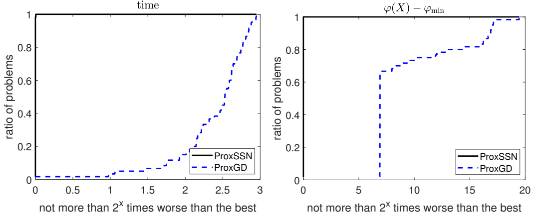
Figure 9: The performance profiles on nonnegative PCA problem (5).
