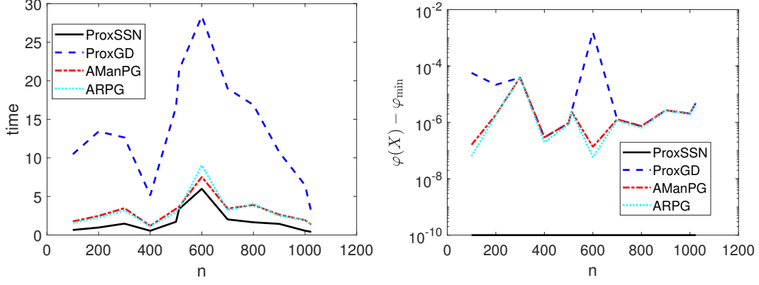
Figure 2: Comparisons of wall-clock time and the objective function values on the sparse PCA problem (3) with p = 20 , \lambda = 0.01 for different n .
