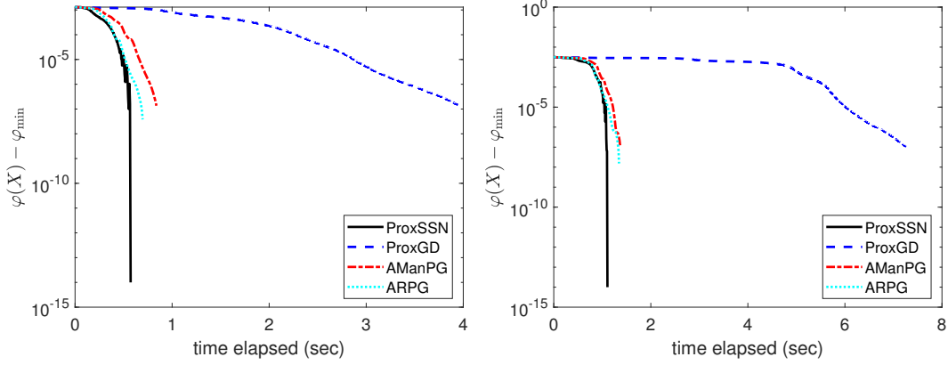
Figure 1: The trajectories of the objective function values with respect to the wall-clock time on the sparse PCA problem (3) with p = 10, \lambda = 0.01 . Left: n = 300 ; right: n = 400
