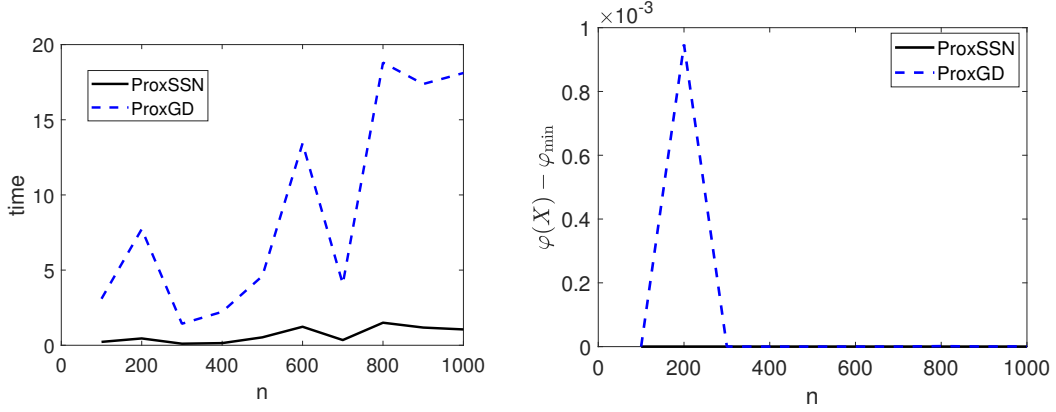
Figure 8: Comparisons of wall-clock time and the objective function values on the nonnegative PCA problem (5) with p = 20 for different n .
