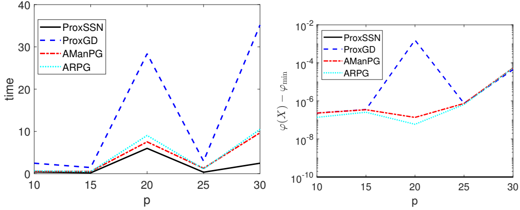
Figure 3: Comparisons of wall-clock time and the objective function values on the sparse PCA problem (3) with n = 512 , \lambda = 0.01 for different p .
