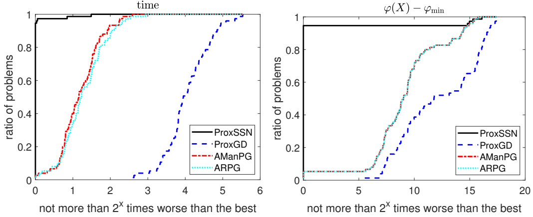
Figure 7: The performance profiles on the sparse least square regression (8).
