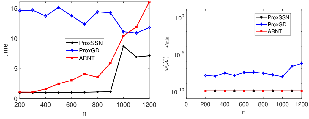
Figure 10: Comparisons of wall-clock time and the objective function values on the BEC problem (39) with \Omega = 0.2 and “b”.
