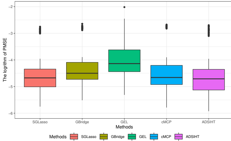
Figure 8: Boxplot of the PMSE.
