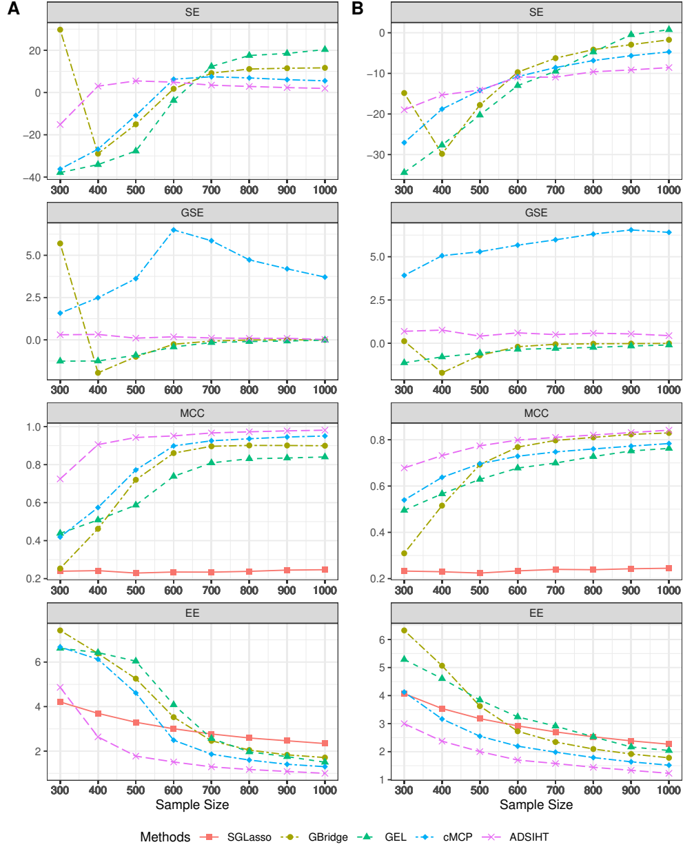
Figure 7: Performance measures as the sample size increases from 300 to 1000. (A) Computational results with homogeneous signal. (B) Computational results with heterogeneous signal.
