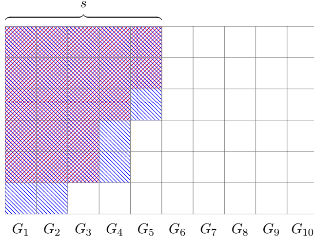
Figure 1: Illustrative example of case 1 . There are 10 groups with equal group size d = 6 , and we reshape the group structure as a 6 \times 10 matrix with each column representing a group. Here s = 5 and s_0 = 4 . The blue region represents the selected set, and the red region represents a (s, s_0) -shaped subset satisfying that total magnitude exceeds ss_0\lambda^2 . Here the cardinality of the red-colored set is s \times s_0 = 20 . Note that the whole vector of support is reshaped into a matrix with a particular group structure.
