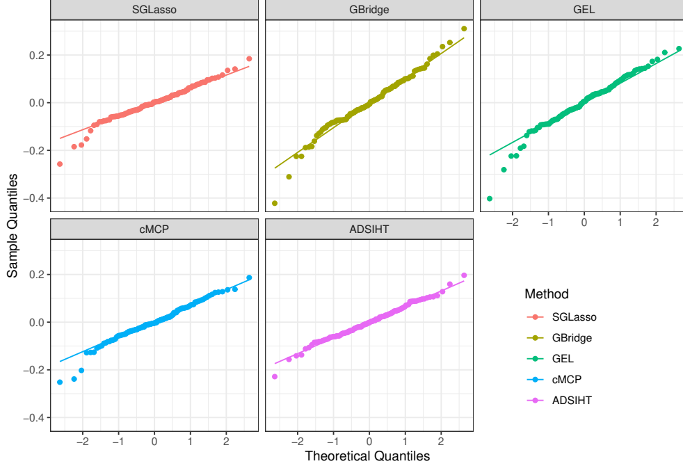
Figure 9: QQ-plots of the residuals.
