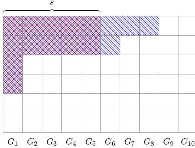
Figure 2: Illustrative example of case 2 . The elements in Figure 2 are the same as in Figure 1. The entries of the red region cover s = 5 groups and its cardinality is less than s \times s_0 = 20 .
