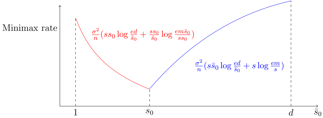
Figure 4: Minimax rate with metric \|\cdot\|_2^2 for different parameter spaces.
