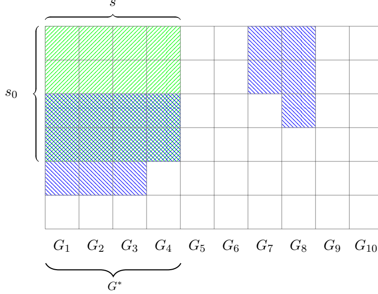
Figure 3: Illustrative example of two cases of false discovery. Here G^* = \{G_1, G_2, G_3, G_4\} and s = s_0 = 4 . The green region represents the true support set S^* and the blue region represents the selected set S^t . The remaining elements in Figure 3 are the same as in Figure 1.
