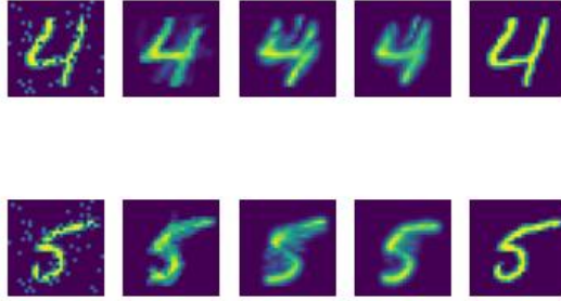
Figure 3: Left to right: image with salt and pepper noise; Euclidean projection; result from Werenski et al. (2022), using optimal weights obtained from their method; result from our approach, using optimal weights obtained from (8); target image.
