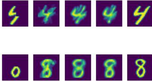
Figure 2: Left to right: occluded image; Euclidean projection; result from Werenski et al. (2022), using optimal weights obtained from their method; result from our approach, using optimal weights obtained from (8); target image.
