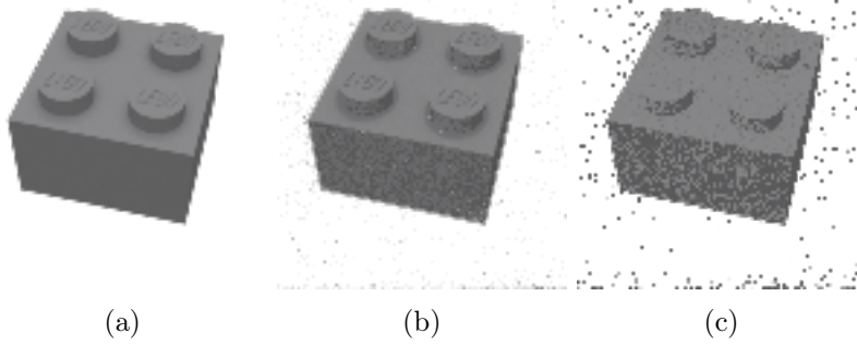
Figure 5: (a) target block, (b) projection from our method, and (c) barycenter obtained from Werenski et al. (2022).
