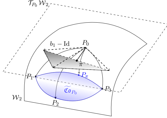
Figure 1: Tangential Wasserstein projection for a general target P_0 .
