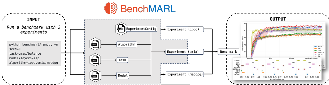
Figure 1: BenchMARL execution diagram. Users run benchmarks as sets of experiments, where each experiment loads its components from the respective YAML configuration files.
