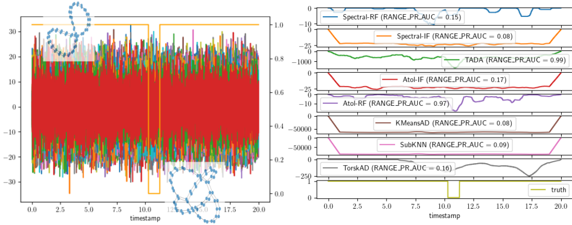
Figure 7: Left: Synthetised time series and the latent generating process (orange) indicating normal connection (double circular wheel with middle connection, on top) or abnormal connection (double circular wheel with two connections, on the bottom). Right: Anomaly scores of all tested methods on one of the data sets, and their RANGE_PR_AUC metric on comparing with the truth (bottom row) in parenthesis.
