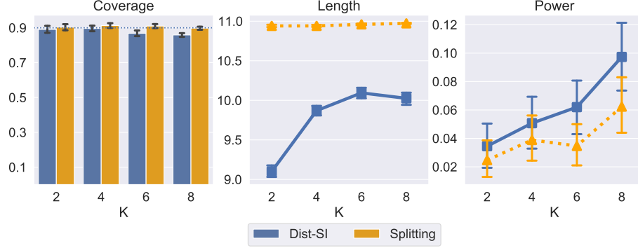
(a) Varying K . Each local machine has \lceil 8000/K \rceil data points for each K .
