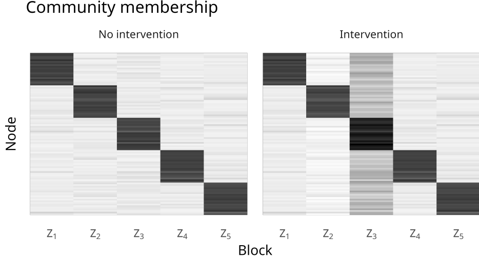
Figure 3: Block memberships in a degree-corrected mixed-membership stochastic blockmodel before and after intervention. Each row corresponds to a node in the network and each column corresponds to a block in the blockmodel. Darker colors indicated increased participation in a given block. The intervention decreases participation in the second community slightly and increases participation in the third community more dramatically. Nodes are sorted by community membership.
