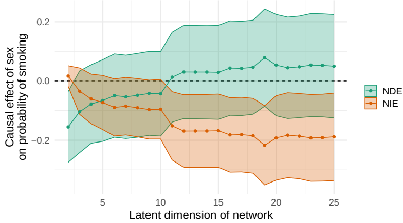
Figure 9: Estimated direct (teal) and indirect (orange) effects of sex on tobacco usage in the Glasgow social network. The estimated effects (vertical axis) vary with the dimension d of the latent space (horizontal axis), and are adjusted for possible confounding by age and church attendance. Positive values indicate a greater propensity for adolescent boys to smoke, while negative values indicate a greater propensity for adolescent girls to smoke.
