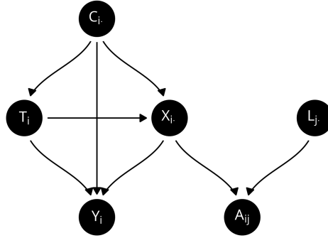
Figure 17: A directed acyclic graph (DAG) representing the causal pathways of latent mediation in a bipartite network. The network has two nodes called i and j and the node i is the unit of interest. Each node in the figure corresponds to a random variable, and edges indicate which random variables may cause which other random variables. We are interested in the causal effect of T_i on Y_i , as mediated by the latent position X_i .
