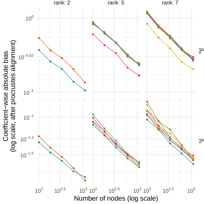
Figure 26: Elementwise bias of \hat{\beta} for \beta under the informative model. This can be thought of as measurement error bias induced by using \hat{X} in place of X . Each column of panels corresponds to a distinct model, where models have varying numbers of latent communities. We visualize results for \hat{\beta}_w and \hat{\beta}_x in separate rows of plots. Within each panel, each line represents results for a single coefficient. Note that the bias disappears asymptotically, as \hat{X} converges to X .
