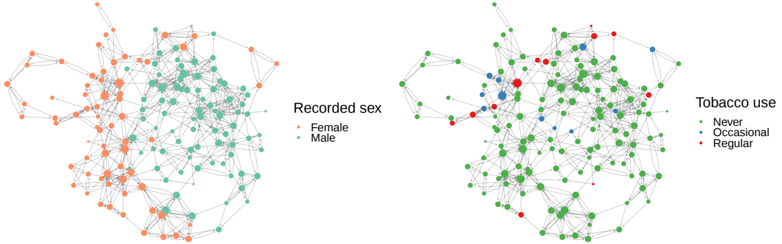
Figure 1: Directed friendships in a secondary school in Glasgow, reported in the Teenage Friends and Lifestyle Study (wave 1). Each node represents one student. An arrow from node i to node j indicates student i claimed student j as a friend. Node size is proportional to in-degree.
