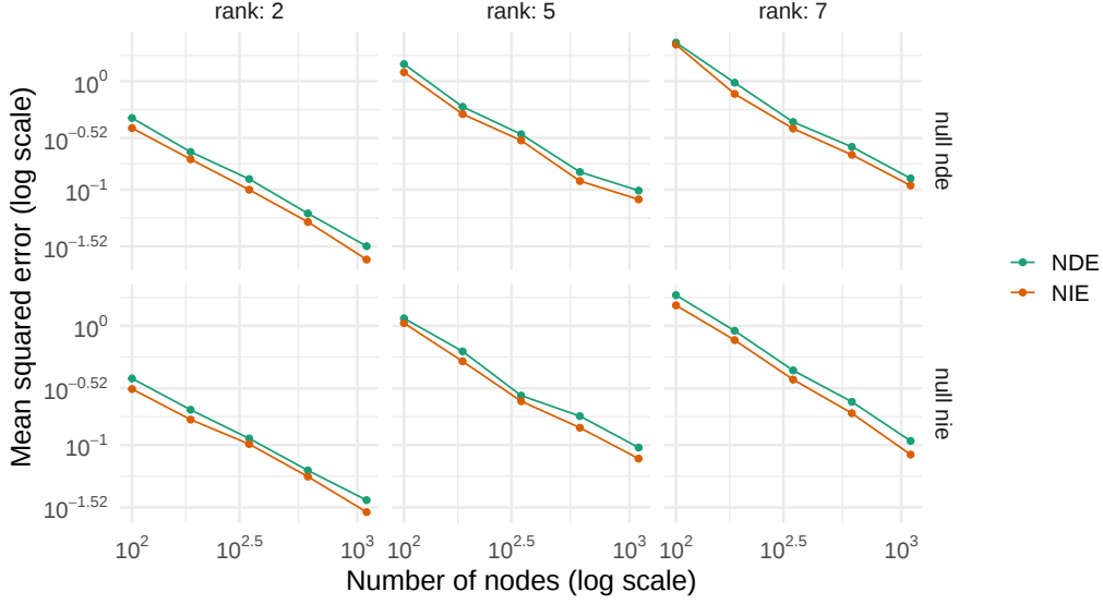
Figure 28: Convergence of \hat{\Psi}_{nde} to \Psi_{nde} and \hat{\Psi}_{nie} to \Psi_{nie} . Each panel shows the mean squared error (vertical axis, log scale) of \hat{\Psi}_{nde} (teal) and \hat{\Psi}_{nie} (orange) as a function of the number of nodes in the network (horizontal axis, log scale). Panels vary horizontally by number of latent communities (left: two blocks, middle: five block, right: seven blocks) and vertically by the simulation model (top: informative, bottom: uninformative).
