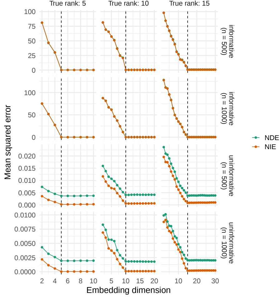
Figure 27: Mean squared error of \hat{\Psi}_{\text{nde}} and \hat{\Psi}_{\text{nie}} when the dimension d is misspecified. Each panel shows mean squared error (vertical axis) of \Psi_{\text{nde}} (teal) and \Psi_{\text{nie}} (orange) as a function of the embedding dimension d (horizontal axis). The dashed vertical line denotes the true latent dimension. Panels vary horizontally by number of latent communities (left: five, middle: ten, right: fifteen) and vertically by the simulation model and number of nodes in the network.
