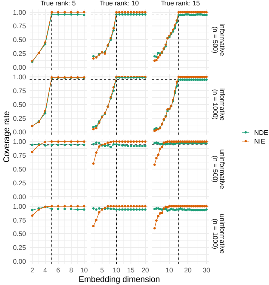
Figure 7: Coverage of confidence intervals for \Psi_{nde} and \Psi_{nie} when the dimension d is misspecified. Each panel shows coverage (vertical axis) of \Psi_{nde} (teal) and \Psi_{nie} (orange) as a function of the embedding dimension d (horizontal axis). The dashed horizontal line denotes the nominal coverage rate of 95% and the dashed vertical line denotes the true latent dimension. Panels vary horizontally by number of latent communities (left: five, middle: ten, right: fifteen) and vertically by the simulation model and number of nodes in the network.
