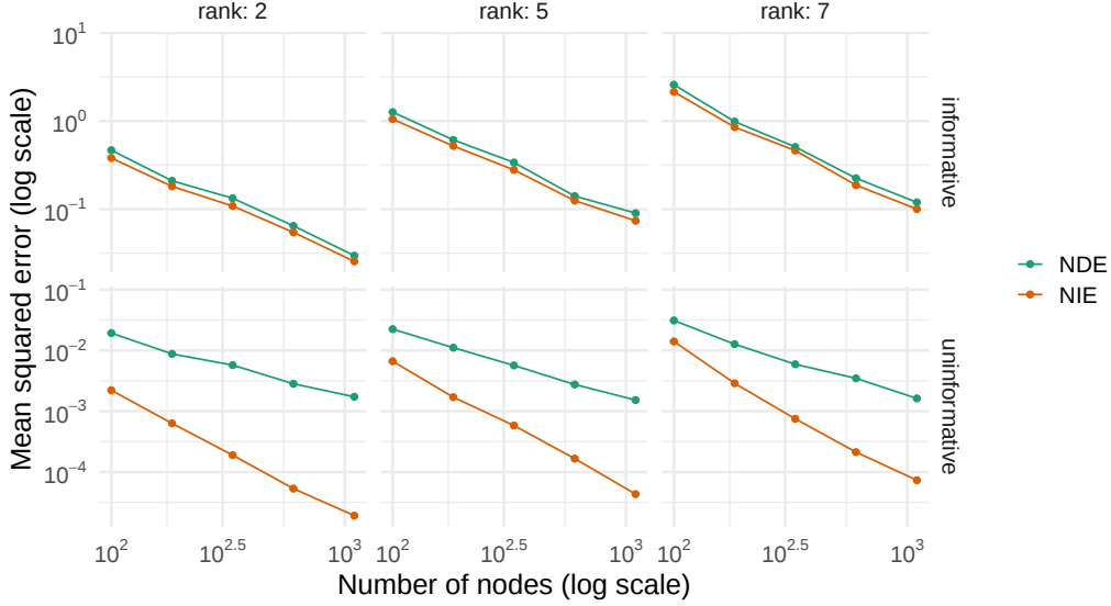
Figure 5: Convergence of \hat{\Psi}_{nde} to \Psi_{nde} and \hat{\Psi}_{nie} to \Psi_{nie} . Each panel shows the mean squared error (vertical axis, log scale) of \hat{\Psi}_{nde} (teal) and \hat{\Psi}_{nie} (orange) as a function of the number of nodes in the network (horizontal axis, log scale). Panels vary horizontally by number of latent communities (left: two blocks, middle: five block, right: seven blocks) and vertically by the simulation model (top: informative, bottom: uninformative).
