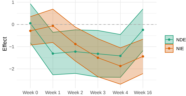
Figure 14: Natural direct and indirect effects of meditation on anxiety level, analyzed independently at each week in the Healthy Minds Trial, controlling for age and sex as confounders, and using a five dimensional embedding of survey responses at each time point.
