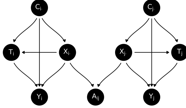
Figure 19: A DAG representing the causal pathways in a network with homophilous confounding , for a network with two nodes called i and j . Compare to Figure 2, where the direction of the X_i \rightarrow T_i and X_j \rightarrow T_j arrows are reversed.
