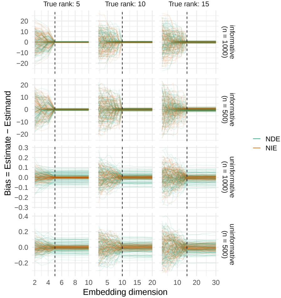
Figure 8: Stability of point estimates for \Psi_{\text{nde}} and \Psi_{\text{nie}} when the dimension d is misspecified. Each panel shows bias (vertical axis) of \hat{\Psi}_{\text{nde}} (teal) and \hat{\Psi}_{\text{nie}} (orange) as a function of the embedding dimension d (horizontal axis). The dashed vertical line denotes the true latent dimension. Panels vary horizontally by number of latent communities (left: five, middle: ten, right: fifteen) and vertically by the simulation model and number of nodes in the network.
