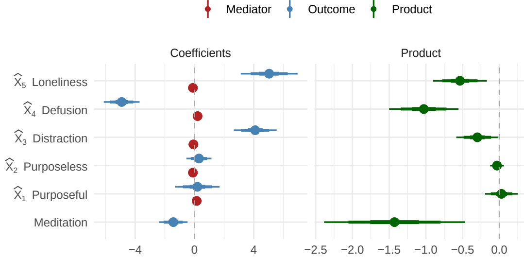
Figure 13: Left: Coefficients from the Healthy Minds mediator and outcome regression models, visualized as point intervals with interval widths 0.5, 0.8, 0.95, respectively. Coefficients for control variables not visualized. Intervals in the mediator model are very close to the point estimates, and thus not visible. All mediator coefficients are statistically distinguishable from zero. Right: confidence intervals for the corresponding coefficient products. The treatment coefficient, labelled “Meditation,” is simply repeated from the left panel for a comparative sense of scale.
