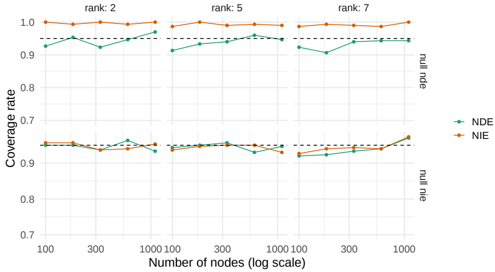
Figure 29: Finite sample coverage of asymptotic confidence intervals for \Psi_{nde} and \Psi_{nie} . Each panel shows coverage (vertical axis) of \Psi_{nde} (teal) and \Psi_{nie} (orange) as a function of the number of nodes in the network (horizontal axis, log scale). The dashed horizontal line denotes the nominal coverage rate of 95%. Panels vary horizontally by number of latent communities (left: two blocks, middle: five block, right: seven blocks) and vertically by the simulation model (top: informative, bottom: uninformative).
