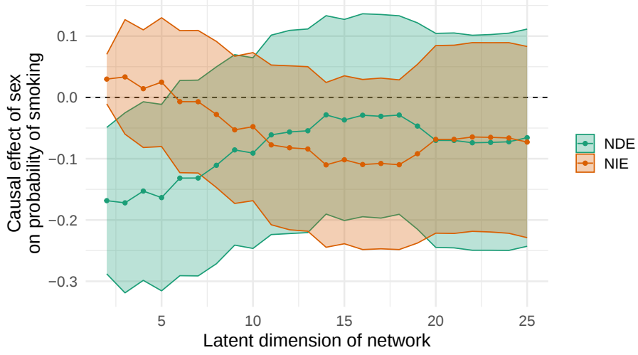
Figure 16: Estimated direct (teal) and indirect (orange) effects of sex on tobacco usage in the Glasgow social network, using the left co-embeddings \hat{X} rather than the right co-embeddings \hat{F} (compare with Figure 9). The estimated effects (vertical axis) vary with the dimension d of the latent space (horizontal axis), and are adjusted for possible confounding by age and church attendance. Positive values indicate a greater propensity for adolescent boys to smoke, while negative values indicate a greater propensity for adolescent girls to smoke.
