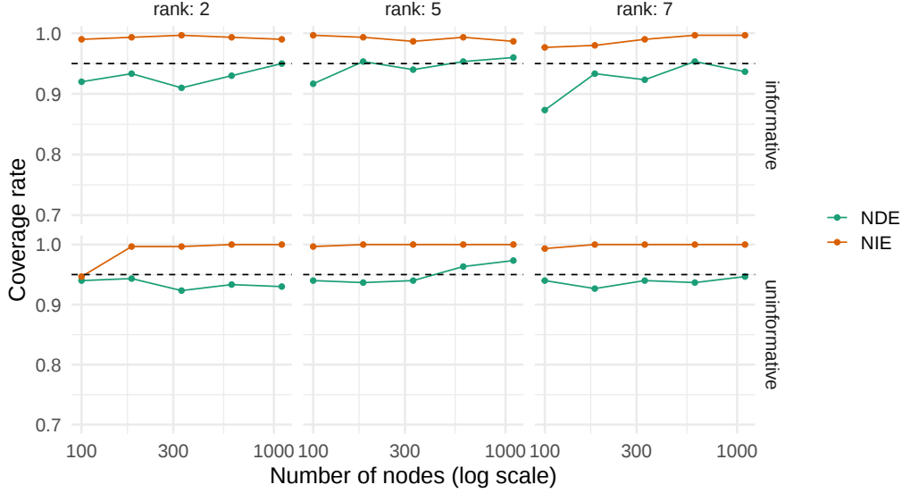
Figure 6: Finite sample coverage of asymptotic confidence intervals for \Psi_{nde} and \Psi_{nie} . Each panel shows coverage (vertical axis) of \Psi_{nde} (teal) and \Psi_{nie} (orange) as a function of the number of nodes in the network (horizontal axis, log scale). The dashed horizontal line denotes the nominal coverage rate of 95%. Panels vary horizontally by number of latent communities (left: two blocks, middle: five block, right: seven blocks) and vertically by the simulation model (top: informative, bottom: uninformative).
