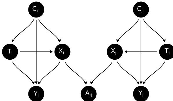
Figure 2: A directed acyclic graph (DAG) representing the causal pathways of latent mediation in a network with two nodes called i and j . Each node in the figure corresponds to a random variable, and edges indicate which random variables may cause which other random variables. We are interested in the causal effect of T_i on Y_i , as mediated by the latent position X_i .
