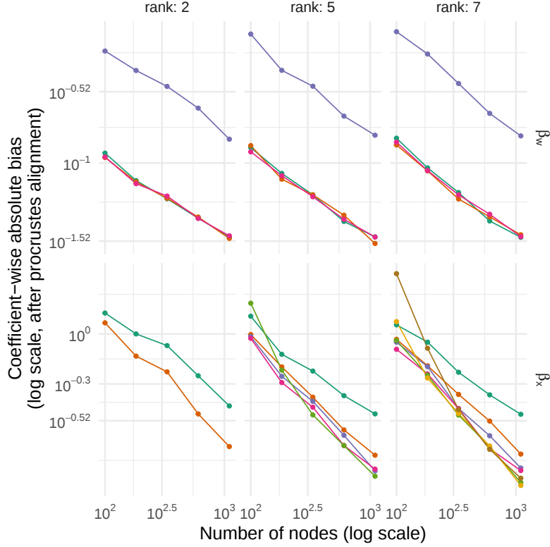
Figure 25: Elementwise bias of \hat{\beta} for \beta under the uninformative model. This can be thought of as measurement error bias induced by using \hat{X} in place of X . Each column of panels corresponds to a distinct model, where models have varying numbers of latent communities. We visualize results for \hat{\beta}_w and \hat{\beta}_x in separate rows of plots. Within each panel, each line represents results for a single coefficient. Note that the bias disappears asymptotically, as \hat{X} converges to X .
