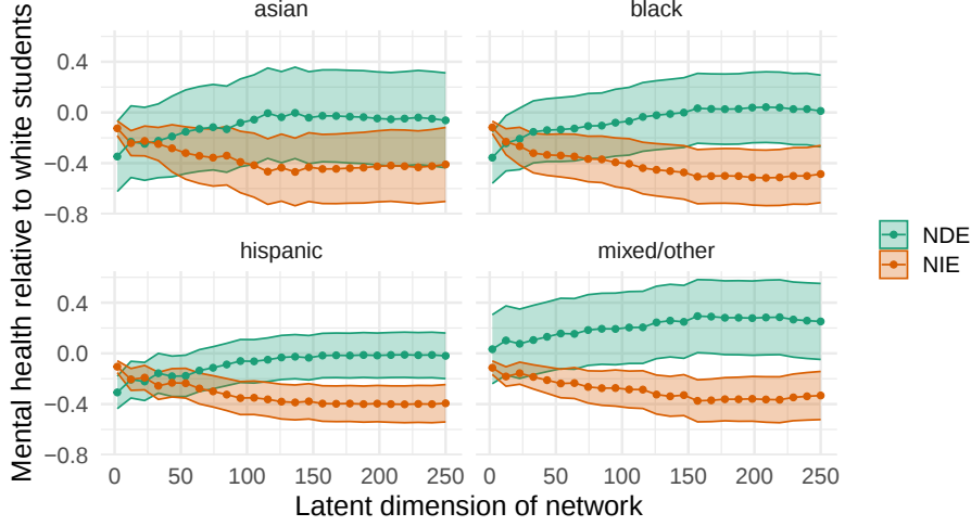
Figure 20: Confidence intervals (95%) for natural direct (teal) and indirect (orange) effects in the AddHealth data example. The vertical axis corresponds to the value of the causal effect, and the horizontal axis encodes the embedding dimension d . All contrasts are relative to white students.
